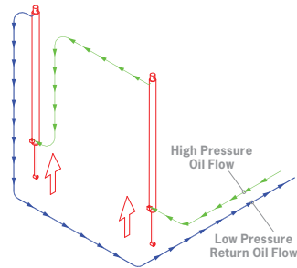
Revolutionary Series Hydraulic Circuit Design
