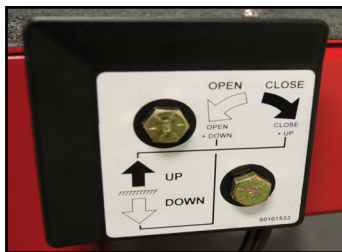
Gravity open, power close
